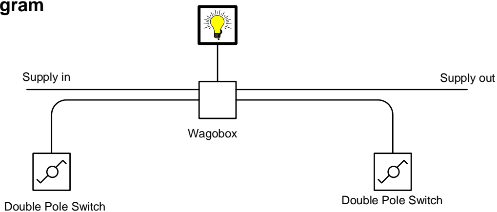
Circuit diagram
