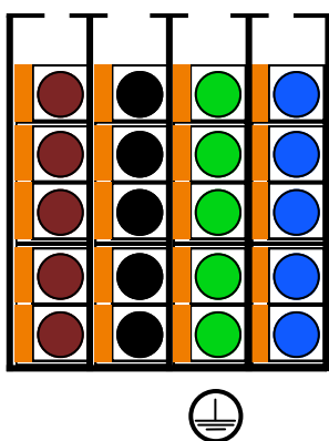
4 Smoke alarms with Interconnect
