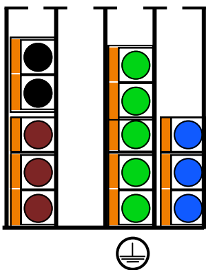
Light Fitting with Switch & Loop
