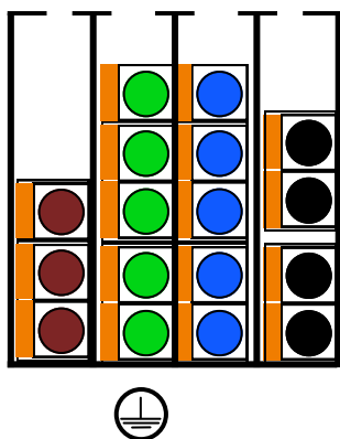
Loop + Switching 2 Separate Loads
