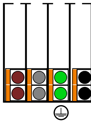
3-Core & Earth Joint
