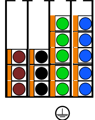
Recessed light with switch + supply loop & S/L Loop
